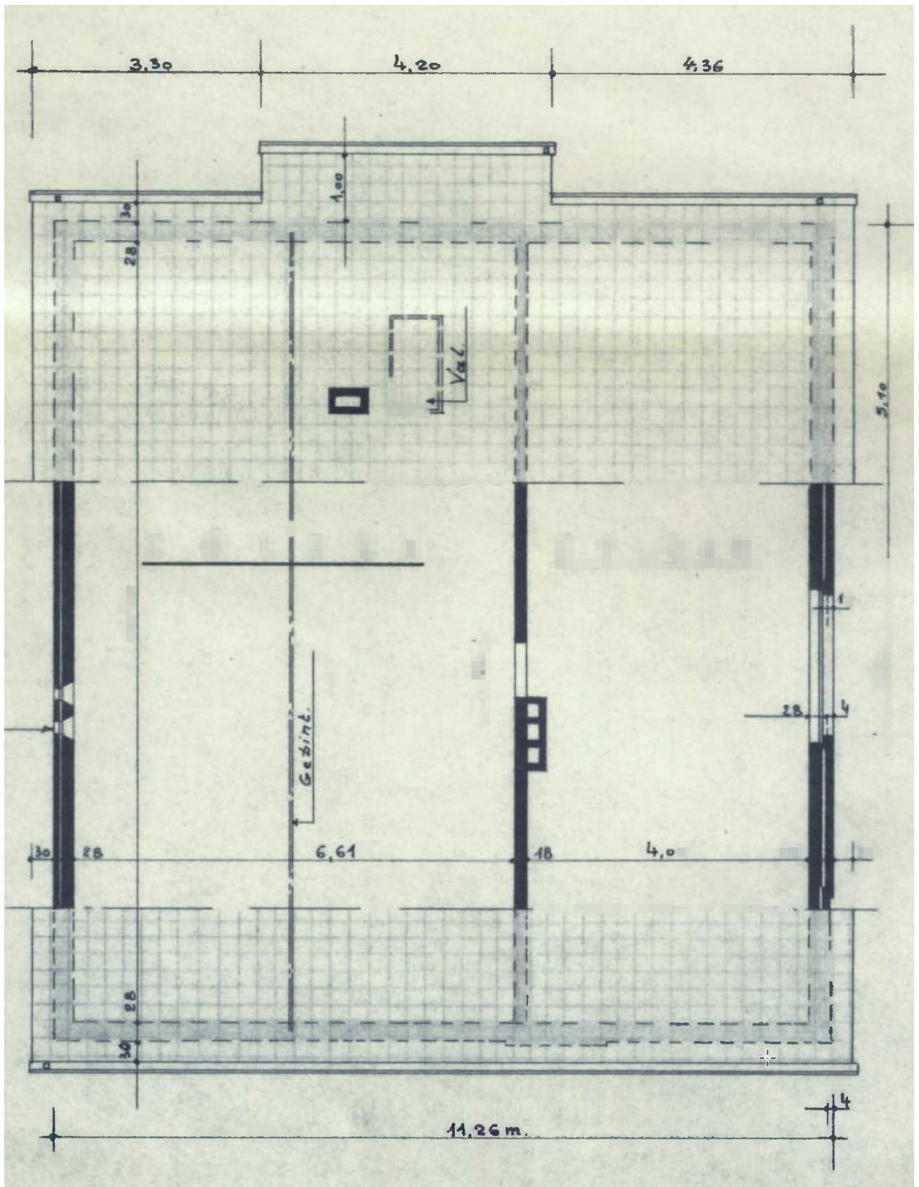
Plan Zolder
