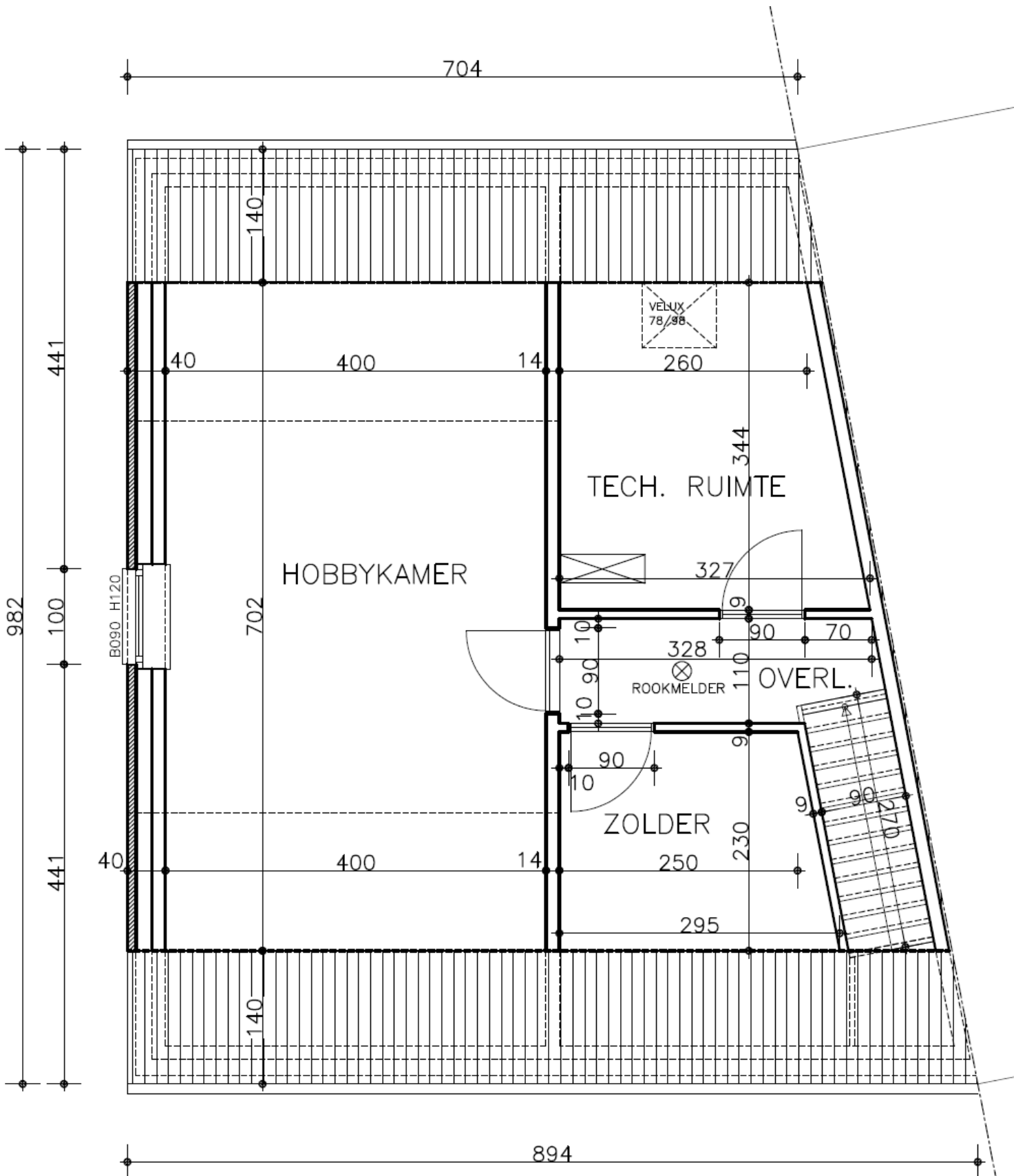
N ZOLDERPLAN sch. 1/50
