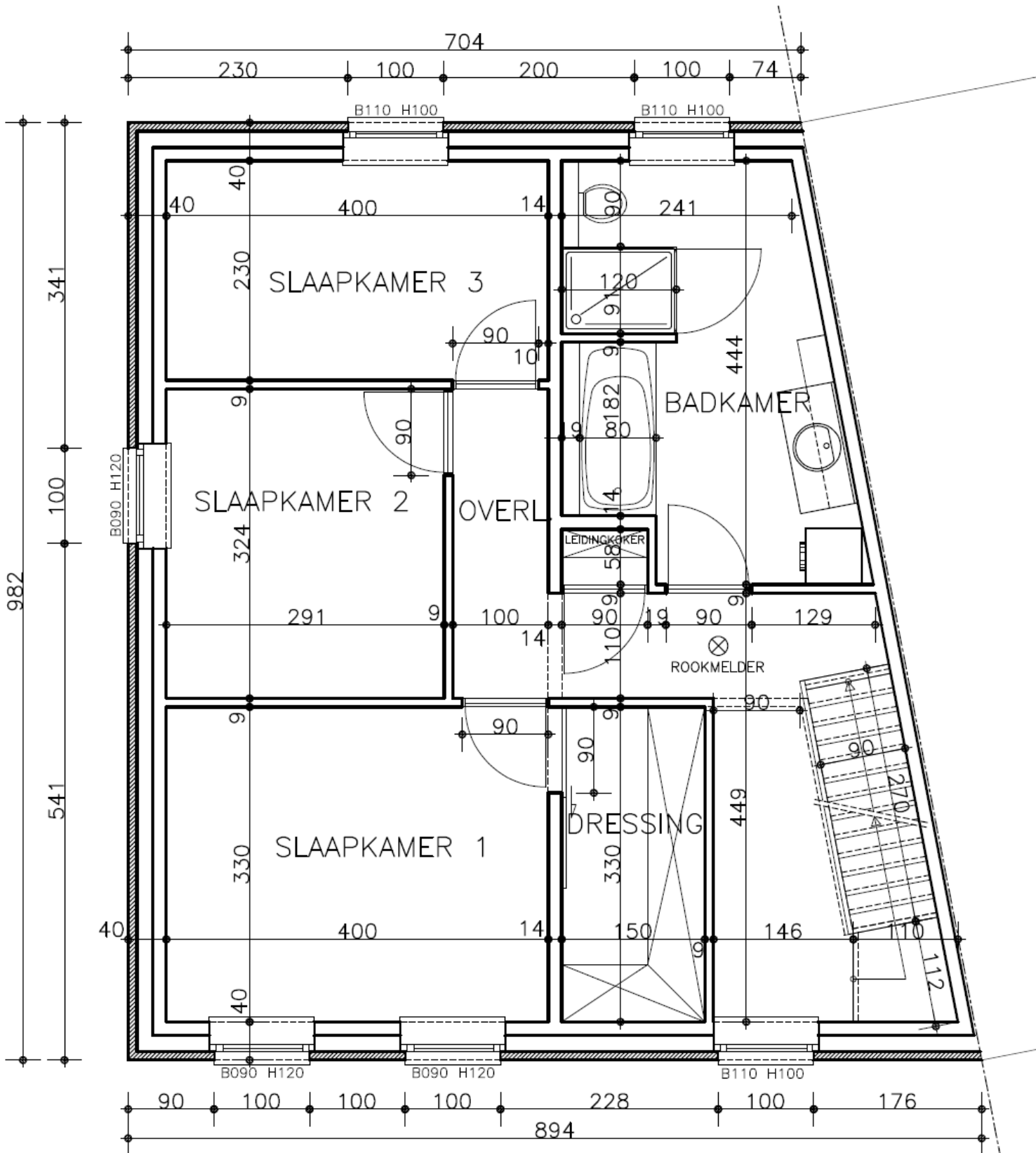
N VERDIEPINGSPLAN sch. 1/50
