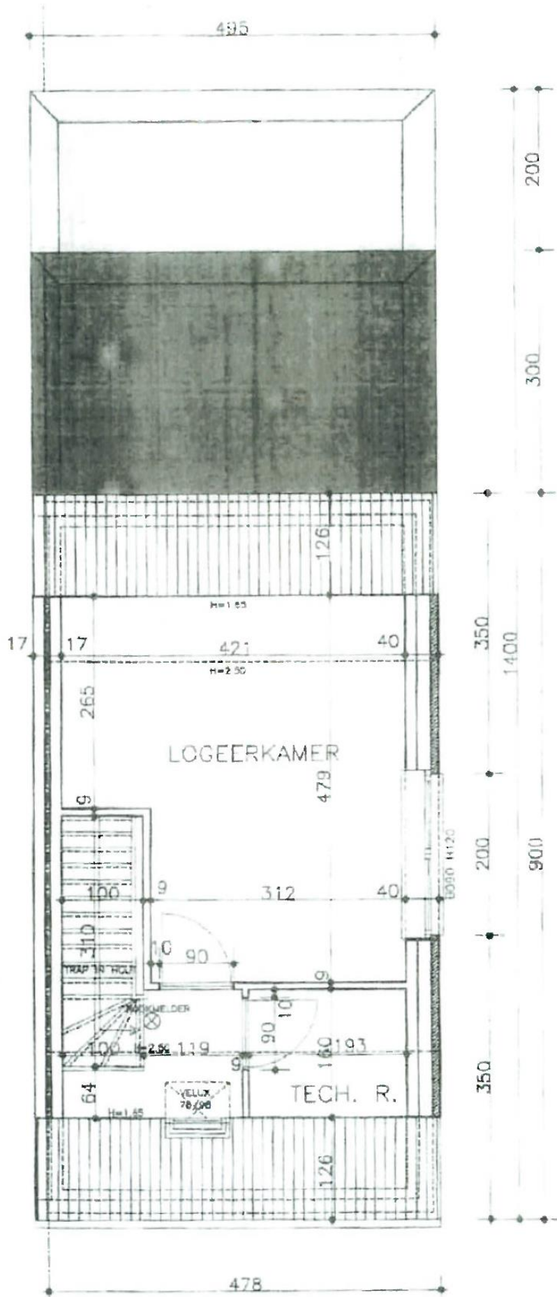
N ZOLDERPLAN sch. 1/50
