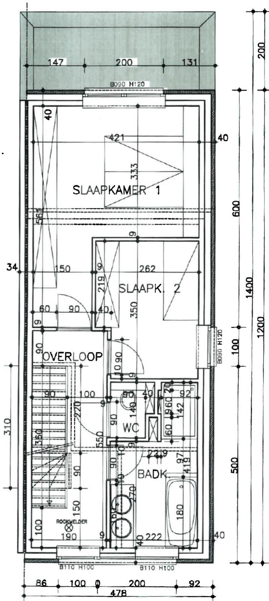
N VERDIEPINGPLAN sch. 1/50
